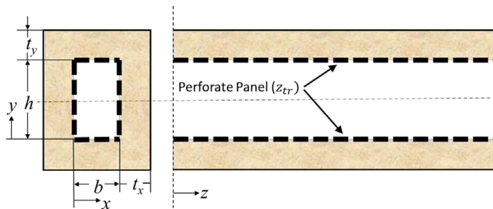
Figure 3.6 Schematic of 4-side Lining Lined Duct
